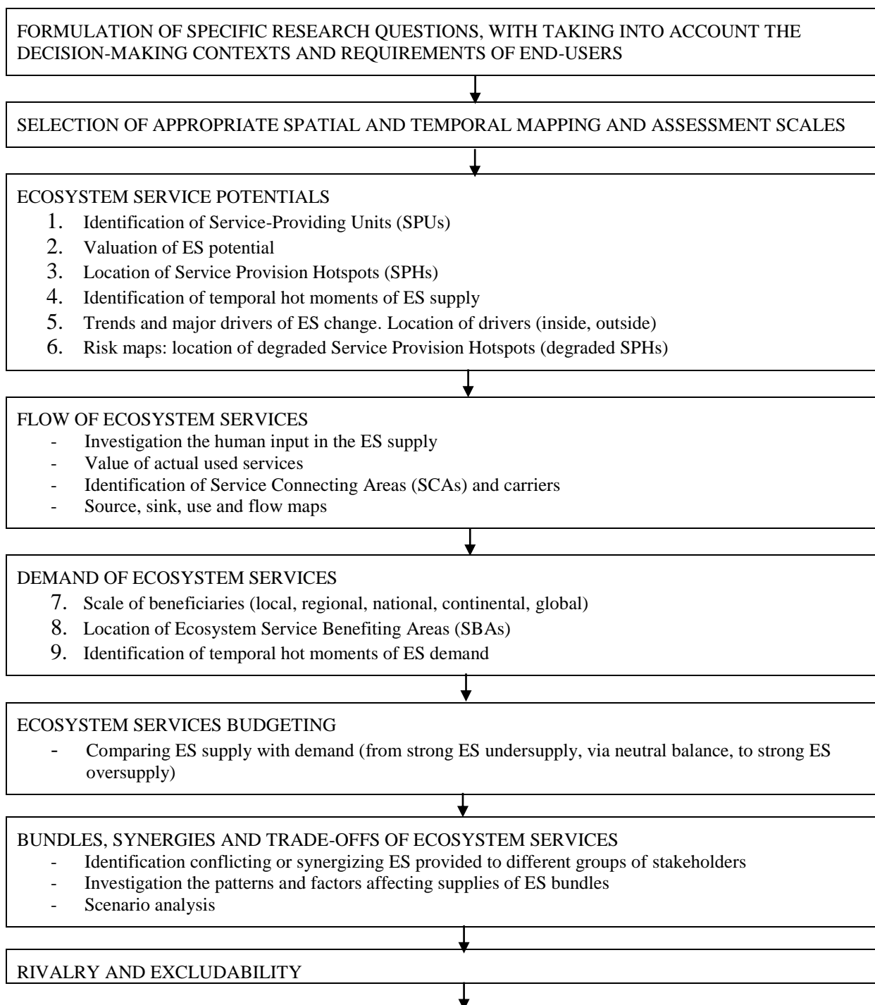
Figure 1. Scope of ecosystem services mapping and assessment.
